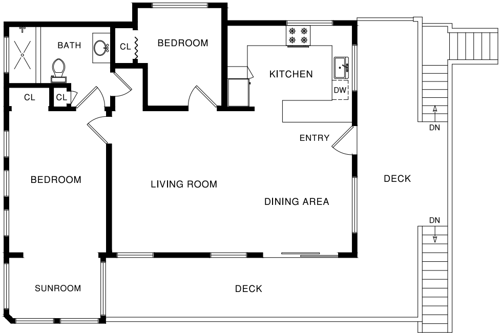
UPPER LEVEL
